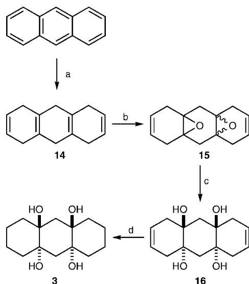
Scheme 3. Reagents and conditions: a) Na, liq. \text{NH}_3 , EtOH, THF, -78\text{ }^\circ\text{C} , 12 h, 80%; b) MCPBA, \text{CH}_2\text{Cl}_2 , -20\text{ }^\circ\text{C} , 5 min, syn/anti = 10:3, 89% overall yield; c) 10% AcOH (aq), 50\text{--}60\text{ }^\circ\text{C} , 6 h, 95%; d) 5% Pd-C, \text{H}_2 , MeOH, 1 h, 95%.
