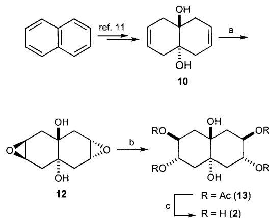
Scheme 2. Reagents and conditions: a) MCPBA, \text{CH}_2\text{Cl}_2 , 0\text{ }^\circ\text{C} \rightarrow room temp., 3 h, 87%; b) i) p TSA, moist DCM, room temp.; ii) \text{Ac}_2\text{O} , pyridine, room temp., 20 h (65% over two steps); c) NaOMe, MeOH, 0\text{ }^\circ\text{C} , 16 h, quant.
